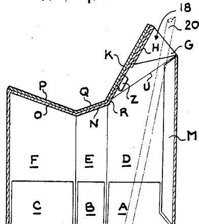
Section 7-7
